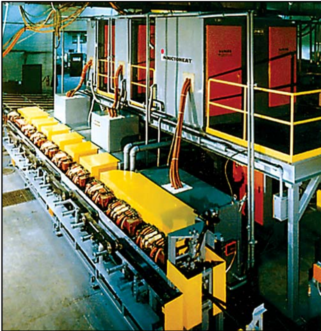
FIGURE 4: Dual frequency (1 kHz and 3kHz) in-line induction steel bar heater
