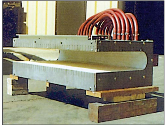
FIGURE 6: Channel coil bar end heater
