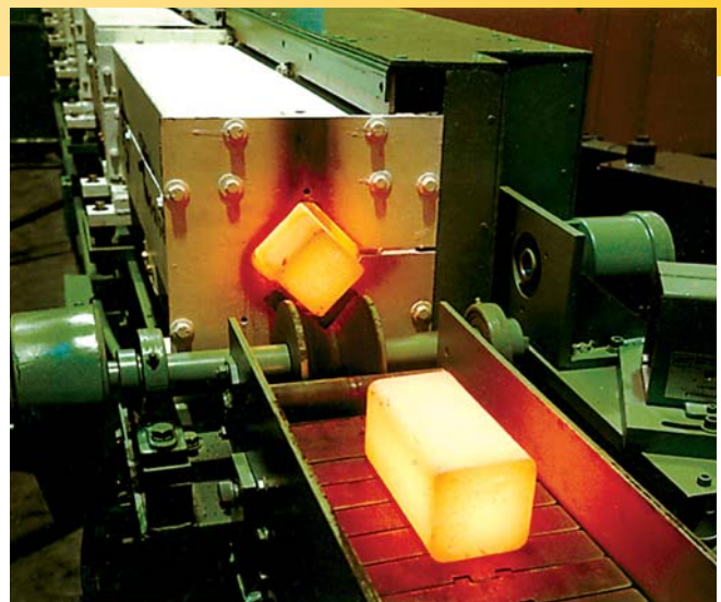
FIGURE 1. Induction heating of round cornered square billets
