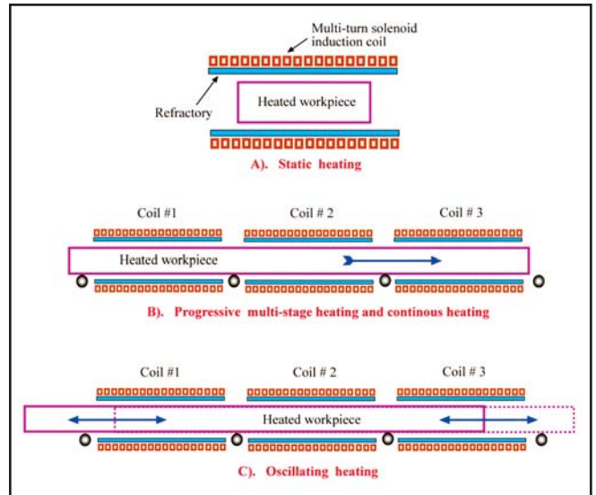
FIGURE 2. Basic heating modes used in induction mass heating
