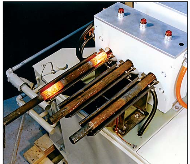
FIGURE 7: Compact induction bar end heater
